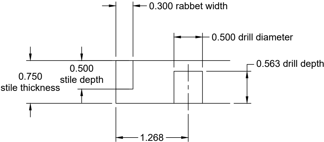
TYPICAL DETAIL Reference - Only machine if displayed.
