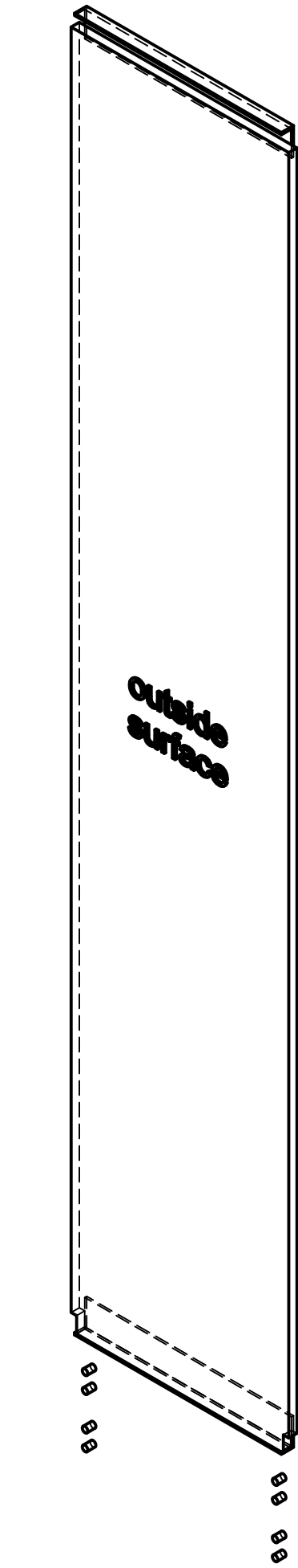
FRONT VIEW Note on drilling and rabbeting Only machine if displayed. Solid circles : machine on the front side Broken circles: machine on the back side
